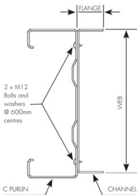
Composite Beam
