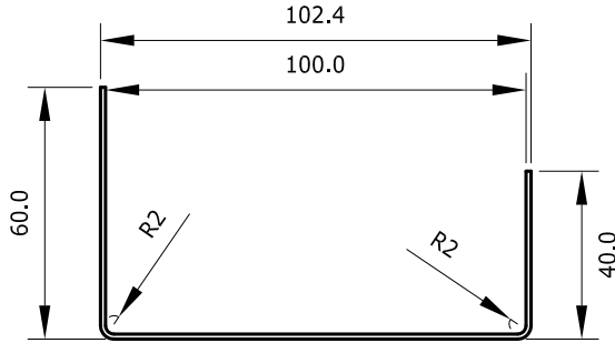
J2 STRIP WIDTH 197.1mm
