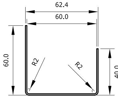
J1 STRIP WIDTH 157.1mm
