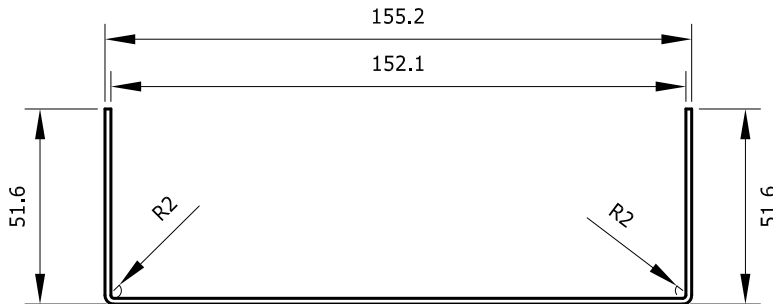
J4 STRIP WIDTH 253.1mm
